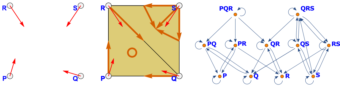
Figure 2. Left: A cloud of vectors. Middle: A possible combinatorial multivector field representation of the cloud of vectors. Right: The associated combinatorial dynamical system represented as a digraph.
