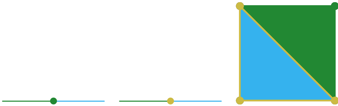
Figure 3. Left: The minimal Morse decomposition of the combinatorial dynamical system in Figure 1(middle) consisting of \{\mathbf{AB}, \mathbf{B}\} (green), and \{\mathbf{BC}\} (blue). Middle: The minimal Morse decomposition of the combinatorial dynamical system in Figure 1(right) consisting of \{\mathbf{AB}\} (green), \{\mathbf{B}\} (yellow), and \{\mathbf{BC}\} (blue). Right: The minimal Morse decomposition of the combinatorial dynamical system in Figure 2(right) consisting of \{\mathbf{P}, \mathbf{Q}, \mathbf{R}, \mathbf{PQ}, \mathbf{PR}, \mathbf{QR}\} (yellow), \{\mathbf{S}, \mathbf{RS}, \mathbf{QS}, \mathbf{QRS}\} (green), and \{\mathbf{PQR}\} (blue).
