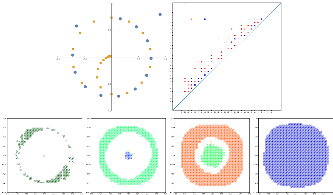
Figure 5. Upper left: two trajectories of (7.1) with starting points at (-0.01, 0.01) (squares) and (0.9, 0.8) (circles). Upper right: persistence diagram for a noisy sampling of (7.1). Red pluses and blue crosses indicate homology generators in dimension zero and one, respectively. Bottom from left to right: Morse sets (randomly colored) in selected filtration steps for threshold values \mu = \frac{48}{148} , \mu = \frac{30}{148} , \mu = \frac{6}{148} , and \mu = \frac{4}{148} , respectively.
