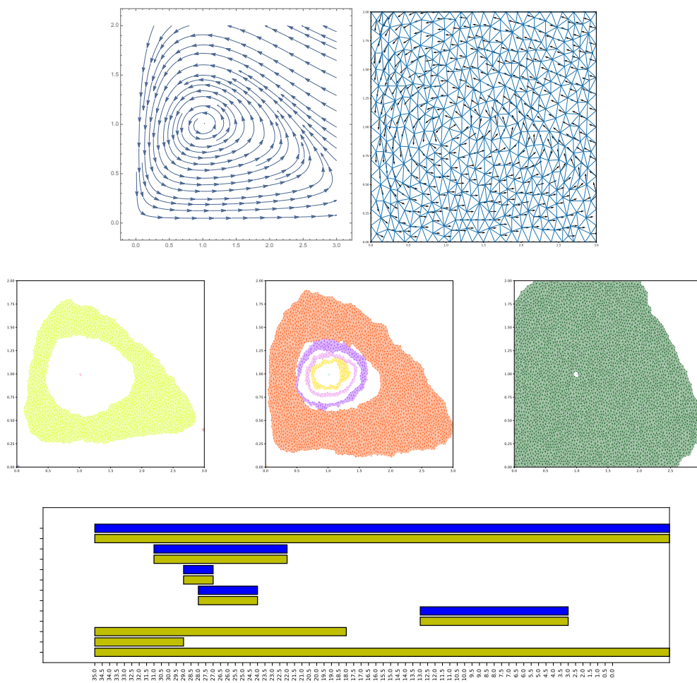
Figure 6. Top: A streamline plot and a cloud of vectors on a triangular grid for the LV model. Middle from left to right: Morse decompositions of combinatorial dynamical systems constructed from the cloud for \alpha = 35^\circ , \alpha = 28^\circ , and \alpha = 0^\circ , respectively. The mesh used contains 4756 points and 9300 triangles. Bottom: The respective persistence barcode. Yellow bars represent generators in dimension 0 and blue bars in dimension 1. The bars are ordered by average size of the Morse sets (biggest on the top).
