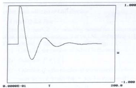
Fig. 18 The output of the PLOTXY( t, e ) statement
