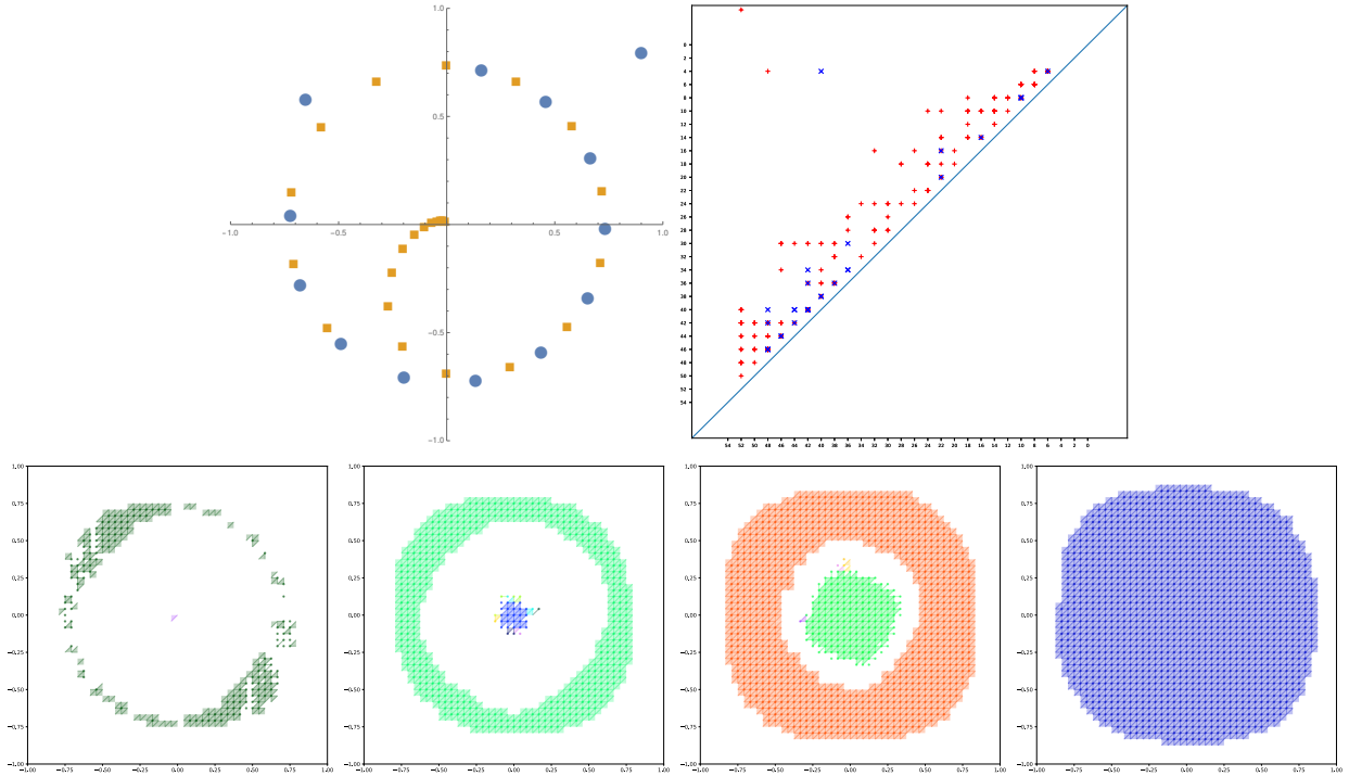
FIGURE 4. Upper left: two trajectories of (7) with starting points at (-0.01, 0.01) (squares) and (0.9, 0.8) (circles). Upper right: persistence diagram for a noisy sampling of (7). Red pluses and blue crosses indicate homology generators in dimension zero and one, respectively. Bottom from left to right: Morse sets in selected filtration steps for threshold values \mu = \frac{48}{148} , \mu = \frac{30}{148} , \mu = \frac{6}{148} and \mu = \frac{4}{148} , respectively.
