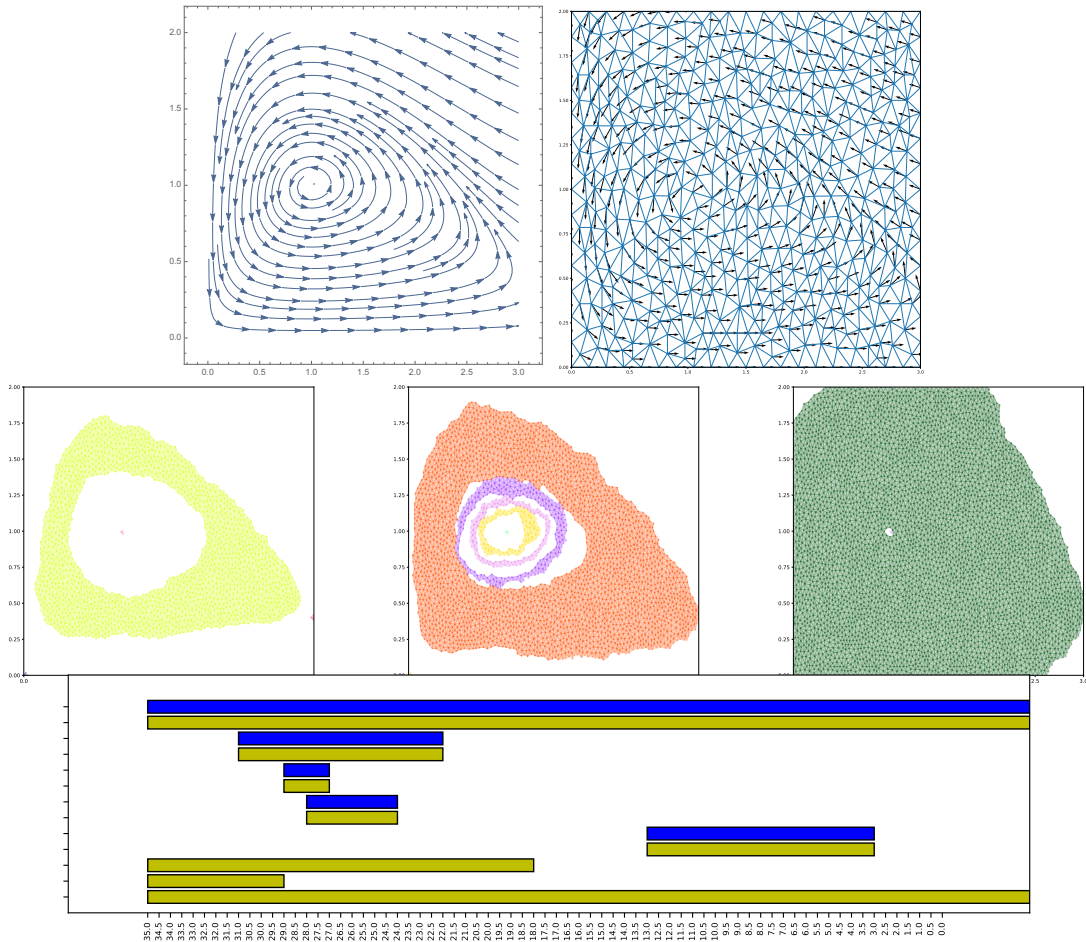
FIGURE 5. Top: A streamline plot and a cloud of vectors on a triangular grid for LV model. Middle from left to right: Morse decompositions of combinatorial dynamical systems constructed from the cloud for \alpha = 35^\circ , \alpha = 28^\circ and \alpha = 0^\circ , respectively. The mesh used contains 4756 points and 9300 triangles. Bottom: The respective persistence barcode. Yellow bars represents generators in dimension 0 and blue bars in dimension 1. The bars are ordered by average size of the Morse sets (biggest on the top).
