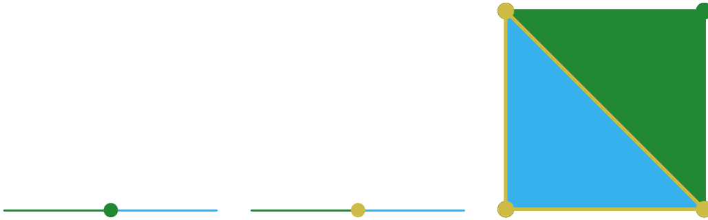
FIGURE 3. Left: The minimal Morse decomposition of the combinatorial dynamical system in Figure 1(middle) consisting of \{\mathbf{AB}, \mathbf{B}\} (green) and \{\mathbf{BC}\} (blue). Middle: The minimal Morse decomposition of the combinatorial dynamical system in Figure 1(right) consisting of \{\mathbf{AB}\} (green), \{\mathbf{B}\} (yellow) and \{\mathbf{BC}\} (blue). Right: The minimal Morse decomposition of the combinatorial dynamical system in Figure 2(right) consisting of \{\mathbf{P}, \mathbf{Q}, \mathbf{R}, \mathbf{PQ}, \mathbf{PR}, \mathbf{QR}\} (yellow), \{\mathbf{S}, \mathbf{RS}, \mathbf{QS}, \mathbf{QRS}\} (green) and \{\mathbf{PQR}\} (blue).
