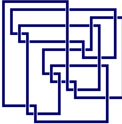
FIGURE 2. Knot K_{14,38437} .
