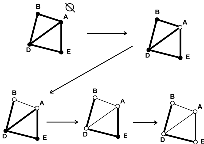
FIGURE 2. Simple coreduction. The missing vertices are marked with circles and the missing edges are marked with thin lines.
